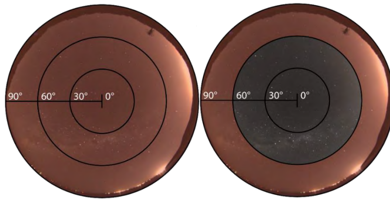
Figure 2: Measurement of mean pixel values; a. Whole-of-sky brightness (full image); b. Horizon brightness (60 – 90°). Shaded areas denote the region of the sky being measured.
